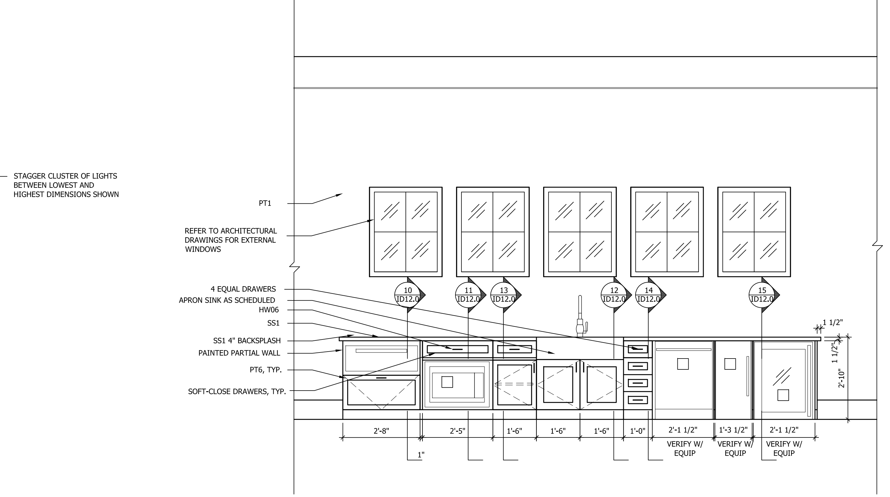
7 CLUB KITCHEN WINDOW WALL ID11.0 SCALE: 1/2" = 1'-0"
