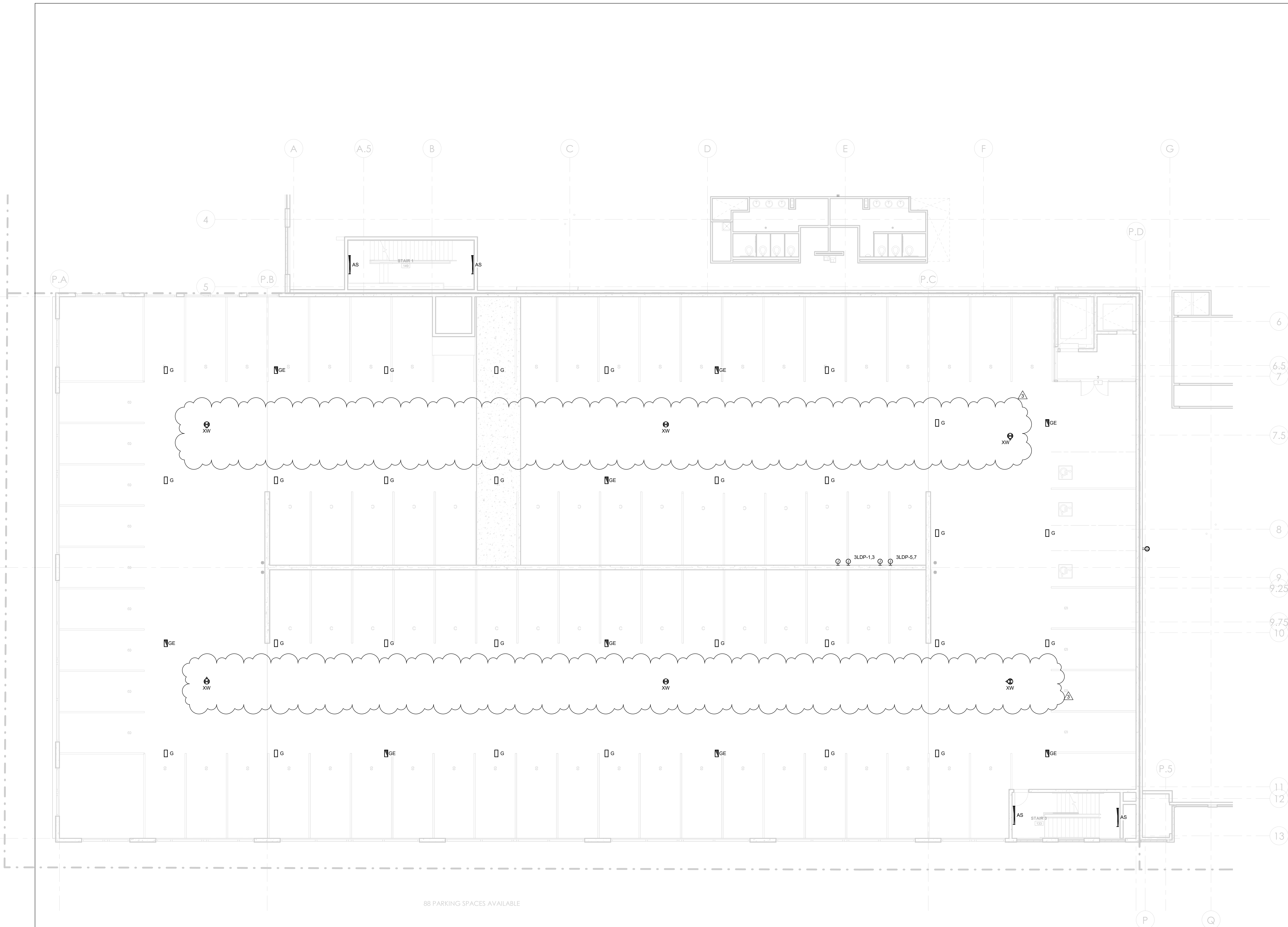
1 PARK LEVEL 3 - ELECTRICAL PLAN EG1.03 SCALE: 1/8" = 1'-0"
