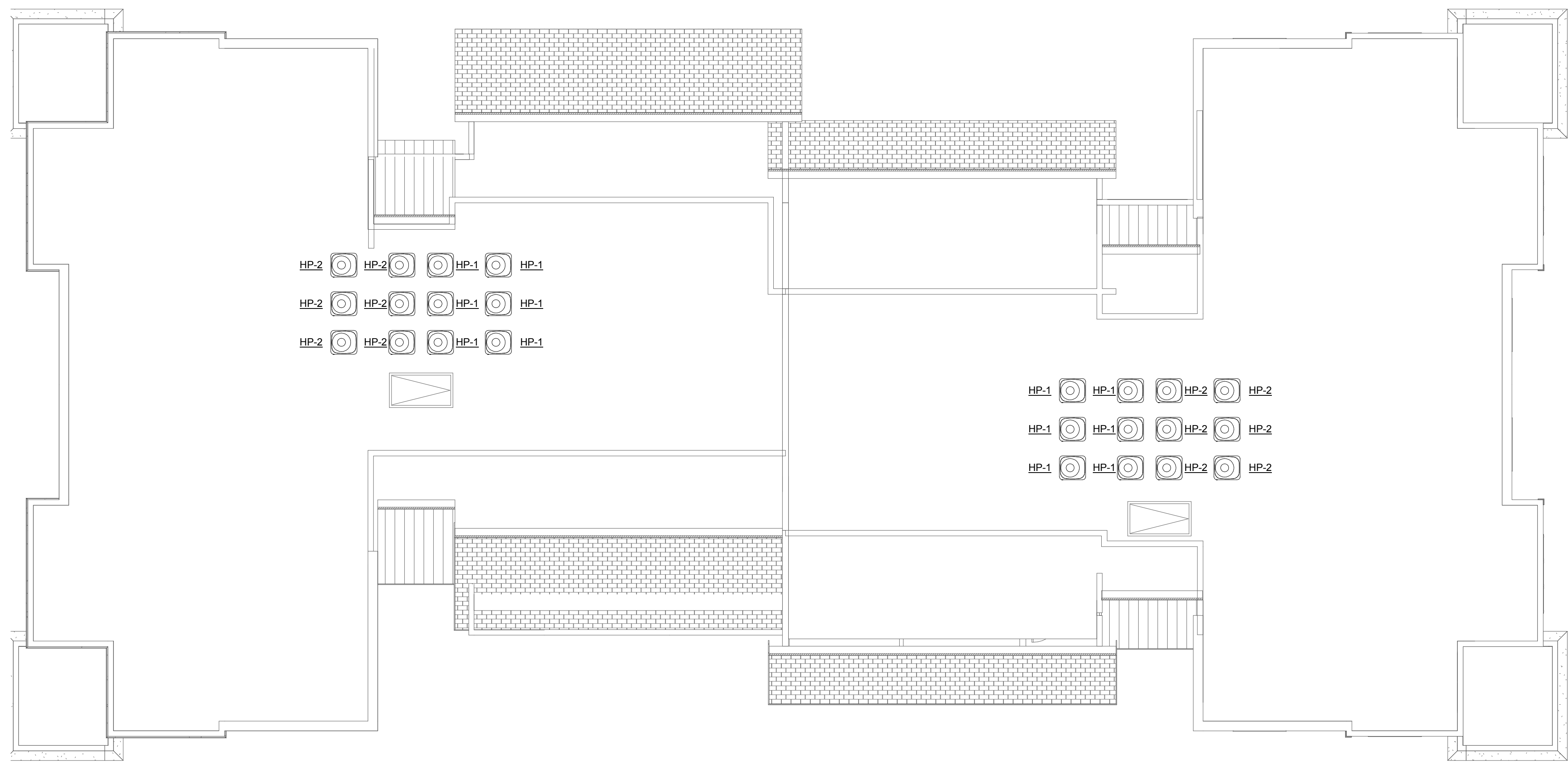
1 M1.22 BLDG TYPE 2 - ROOF PLAN - MECHANICAL SCALE: 1/8" = 1'-0"
