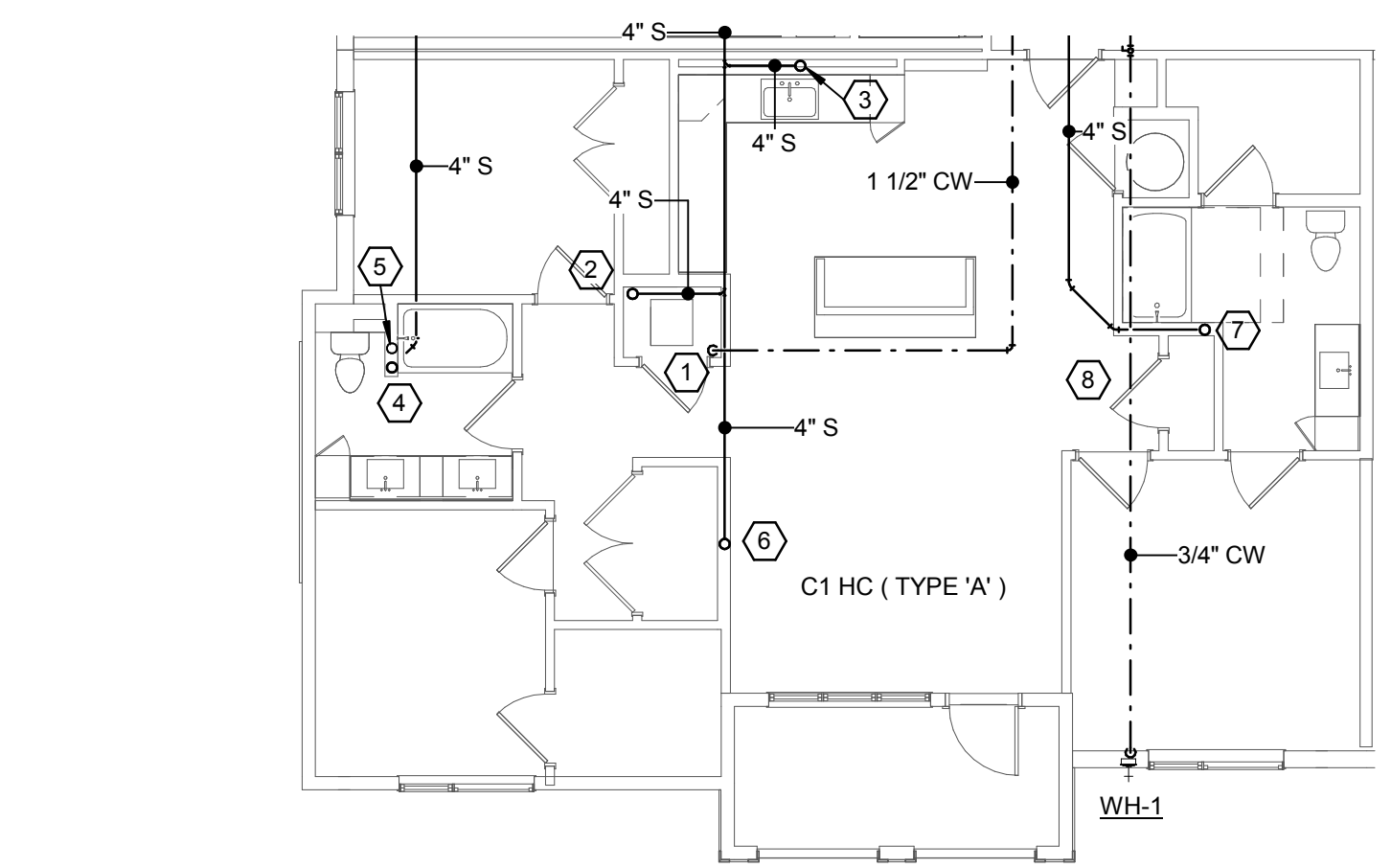
1A BLDG TYPE 1(ALT) - FIRST FLOOR PLAN (PARTIAL) - PLUMBING PT.11 SCALE: 1/8" = 1'-0"
