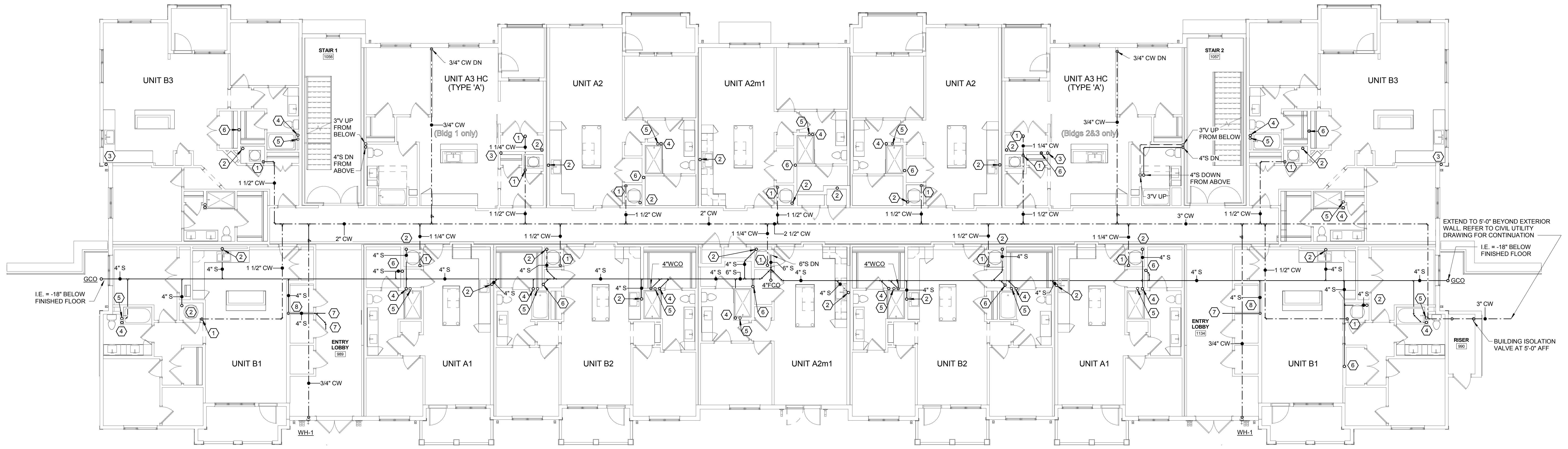
2 BLDG TYPE 2 - SECOND FLOOR PLAN - PLUMBING SCALE: 1/8" = 1'-0"
