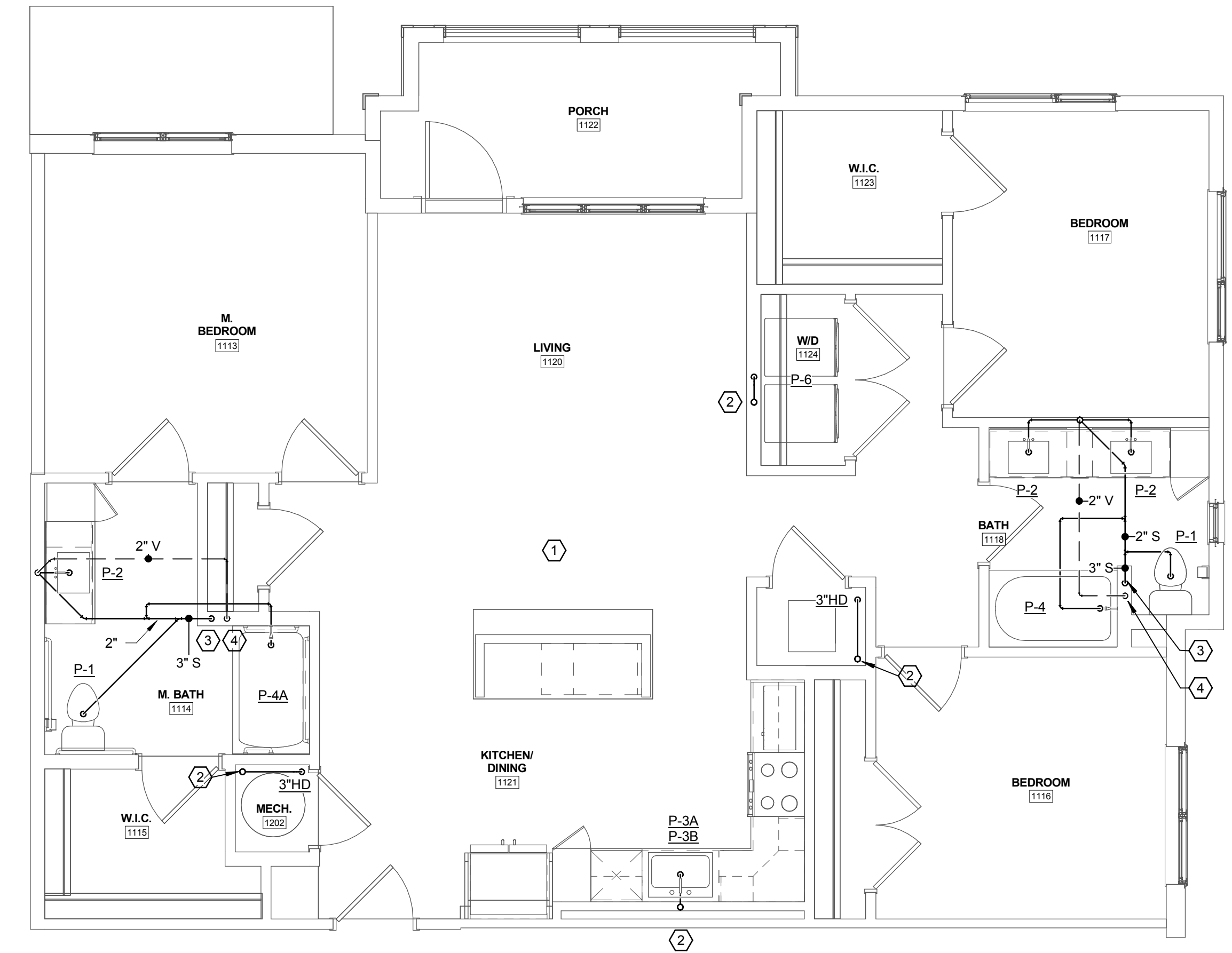
3 UNIT C1-HC (TYPE 'A') - SANT/VENT P4.05 SCALE: 1/4" = 1'-0"
