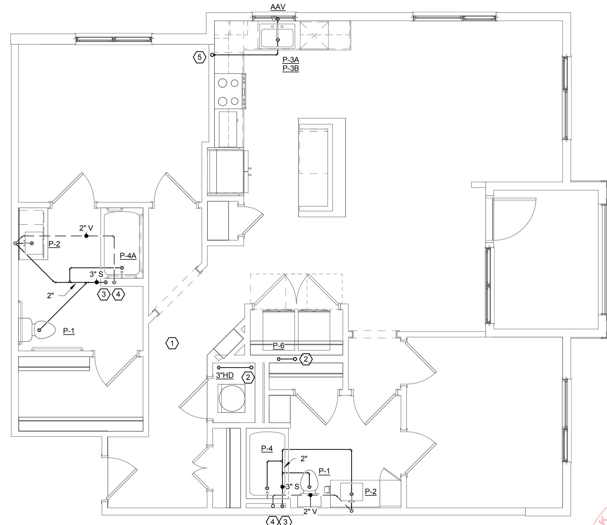
2 UNIT B3-HC (TYPE 'A') - SANT/VENT P4.05 SCALE: 1/4" = 1'-0"
