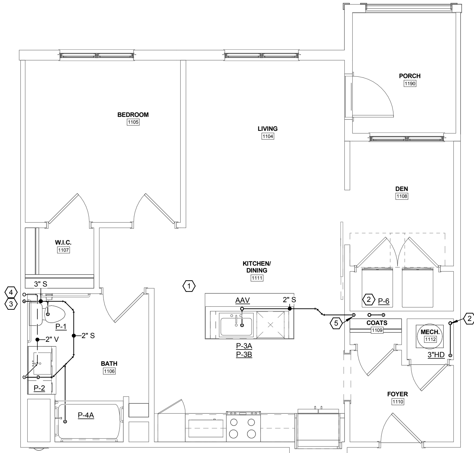
1 UNIT A3-HC (TYPE 'A') - SANT/VENT P4.05 SCALE: 1/4" = 1'-0"
