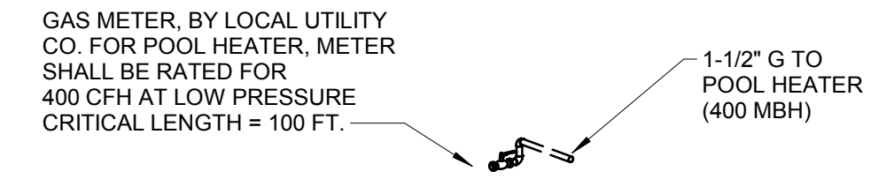
3 Natural Gas Riser Diagram - Maintenance Bldg SCALE:
