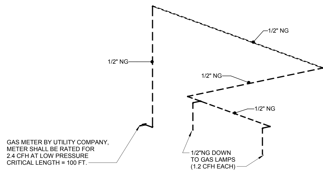
2 Natural Gas Riser Diagram - Leasing Bldg SCALE:
