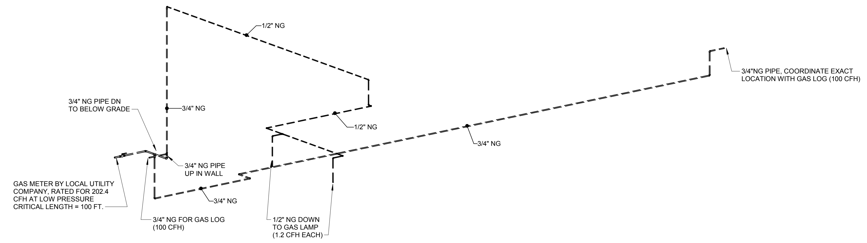
1 Natural Gas Riser Diagram - Club Amenity Bldg SCALE:
