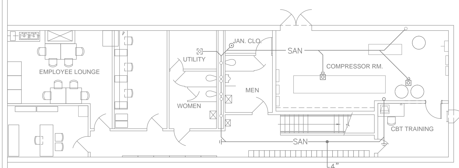
3 MEZZANINE PLAN SCALE: 3/32" = 1'-0"
