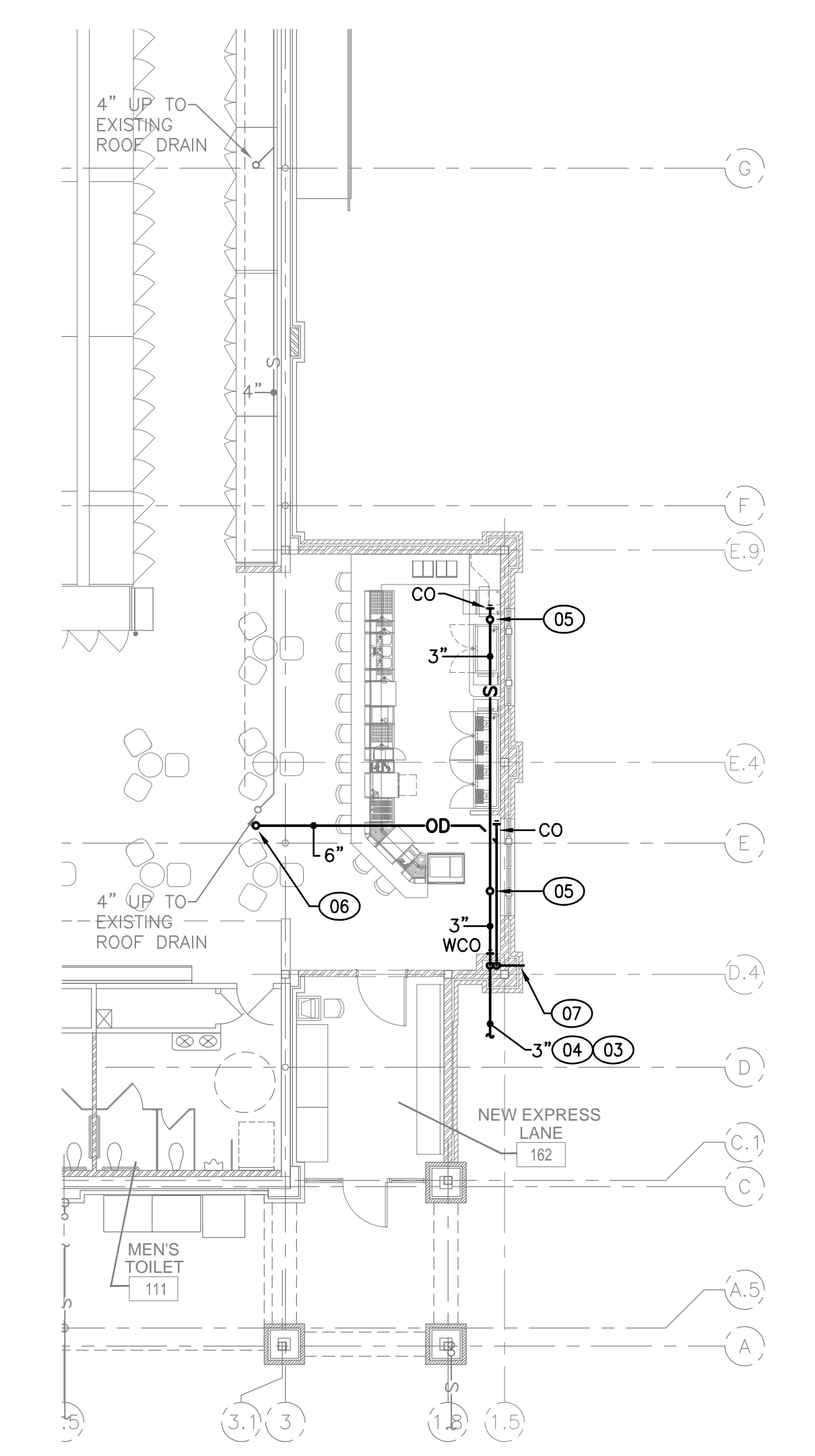
2 PARTIAL STORM PIPING PLAN SCALE: 3/32" = 1'-0"
