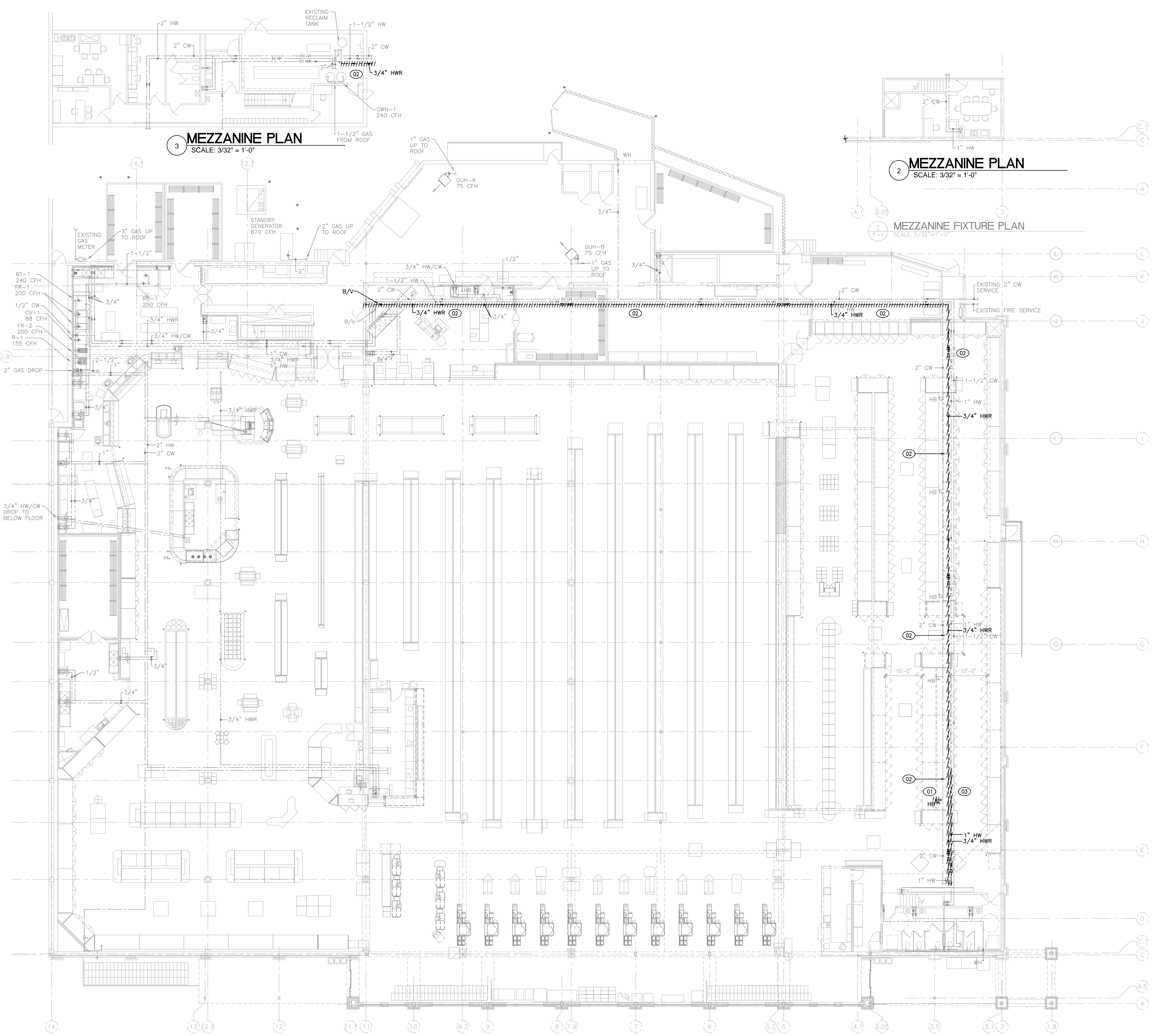
1 PLUMBING WATER AND GAS DEMOLITION PLAN SCALE: 3/32" = 1'-0"
