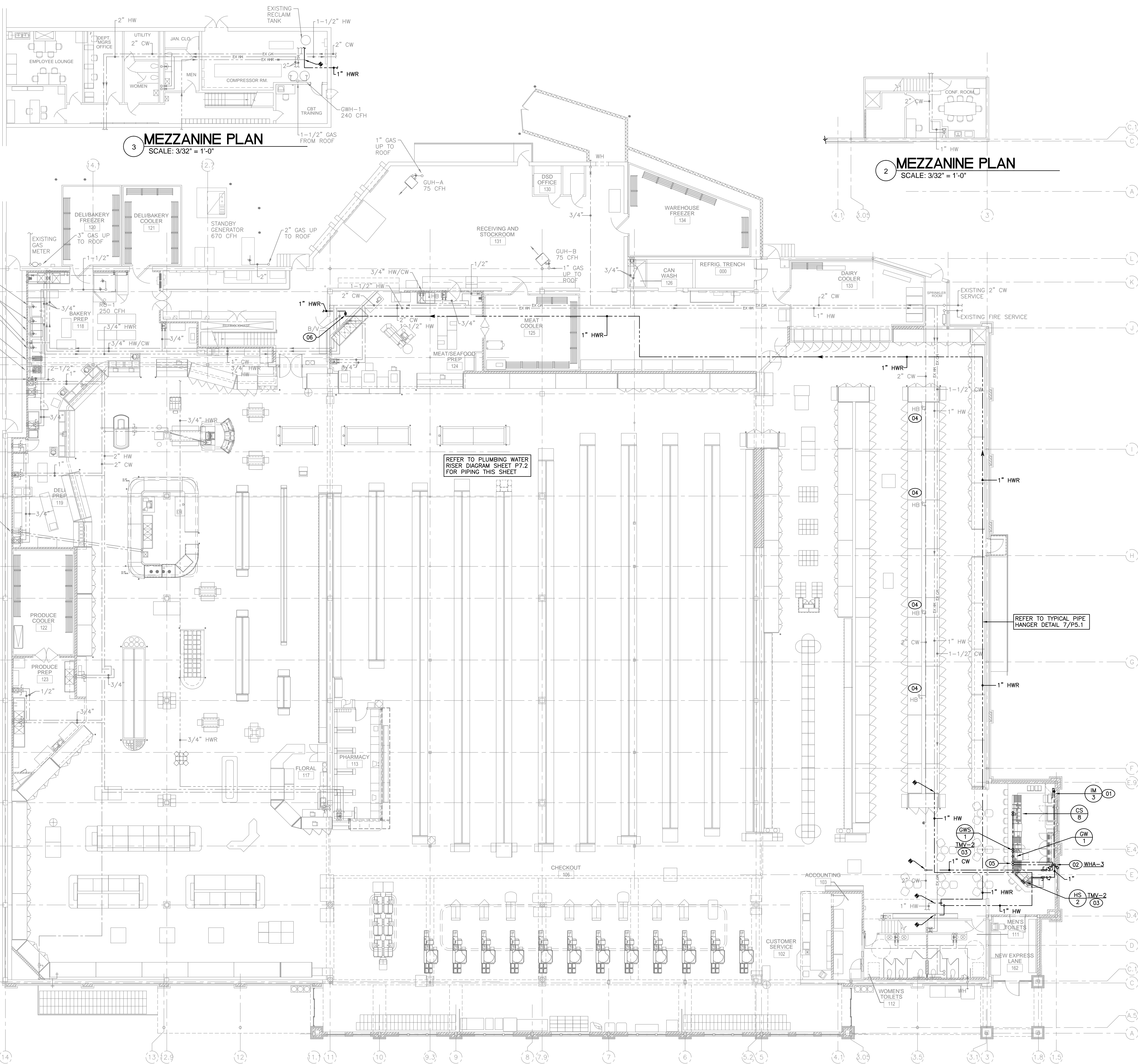
1 PLUMBING WATER AND GAS PIPING PLAN SCALE: 3/32" = 1'-0"
