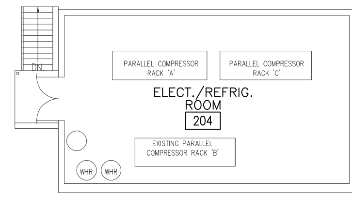
MECH. MEZZANINE PLAN SCALE: 3/32" = 1'-0"
