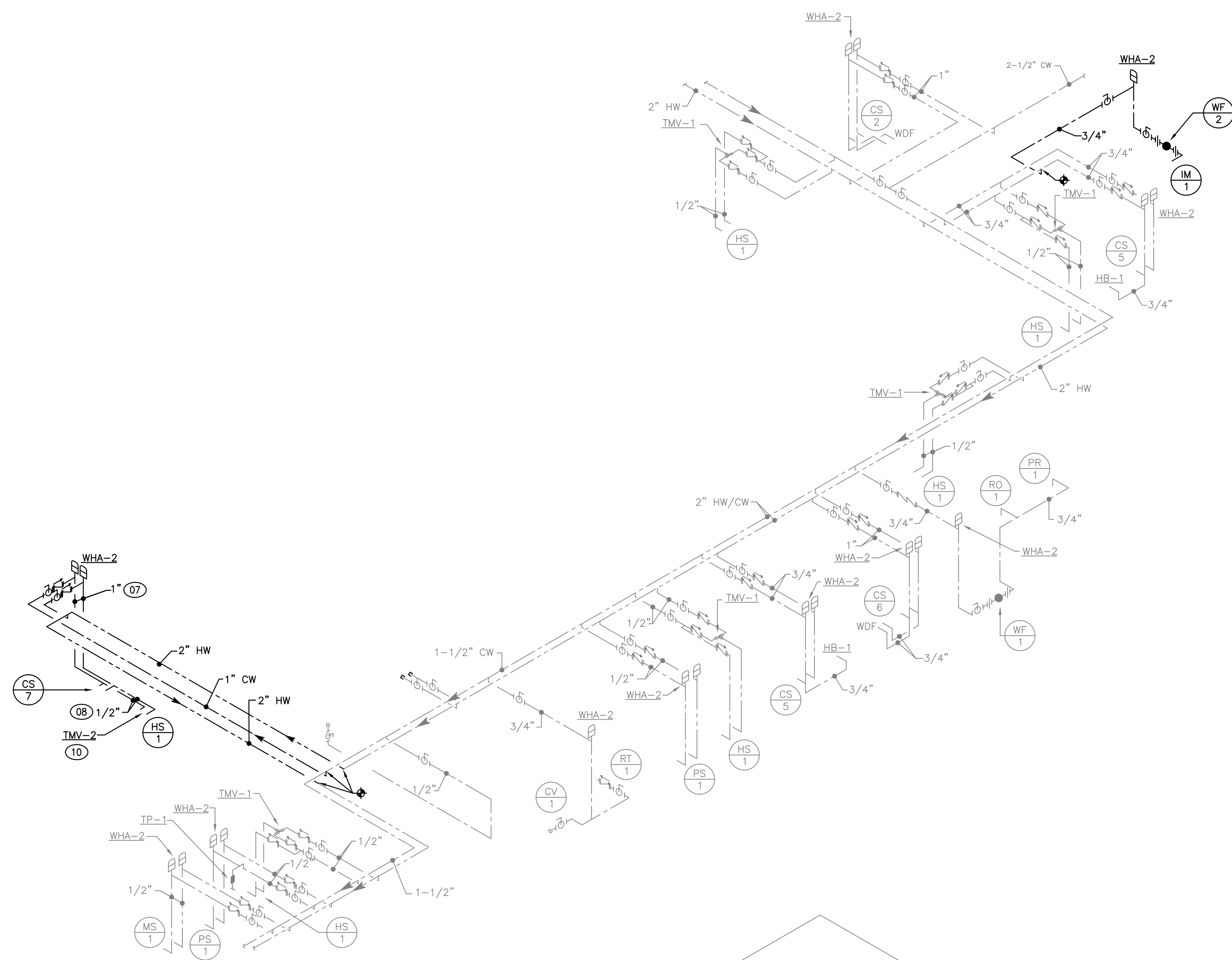
1 PARTIAL WATER RISER DIAGRAM NO SCALE
