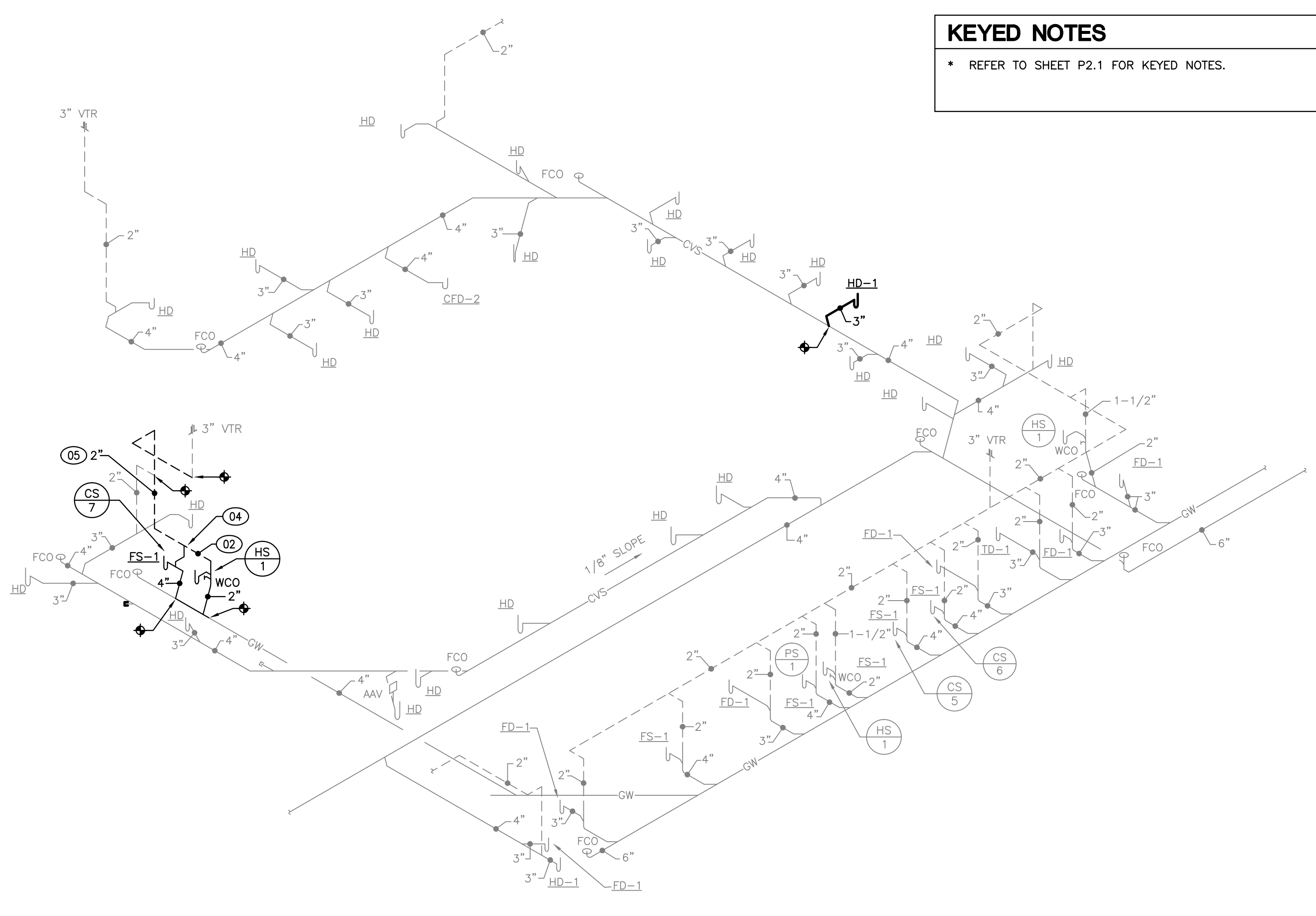
2 PARTIAL DRAINAGE RISER DIAGRAM NO SCALE
