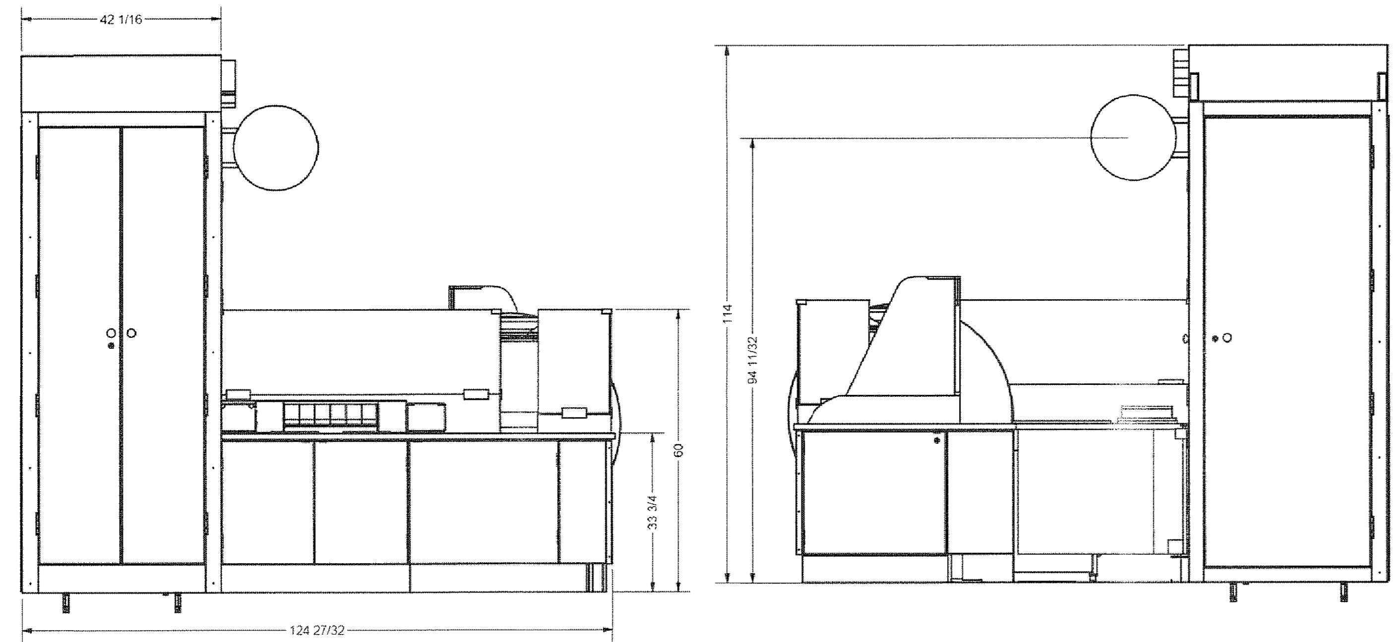
RIGHT ELEVATION VIEW
