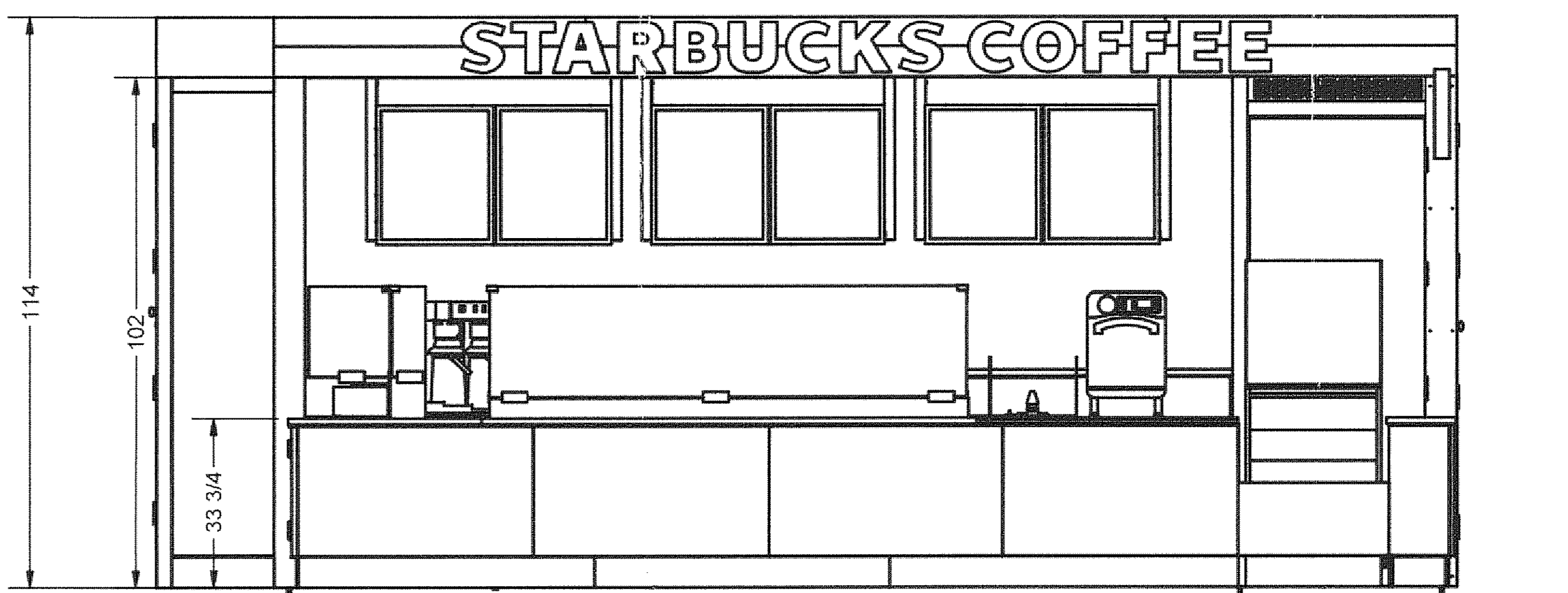
FRONT VIEW
