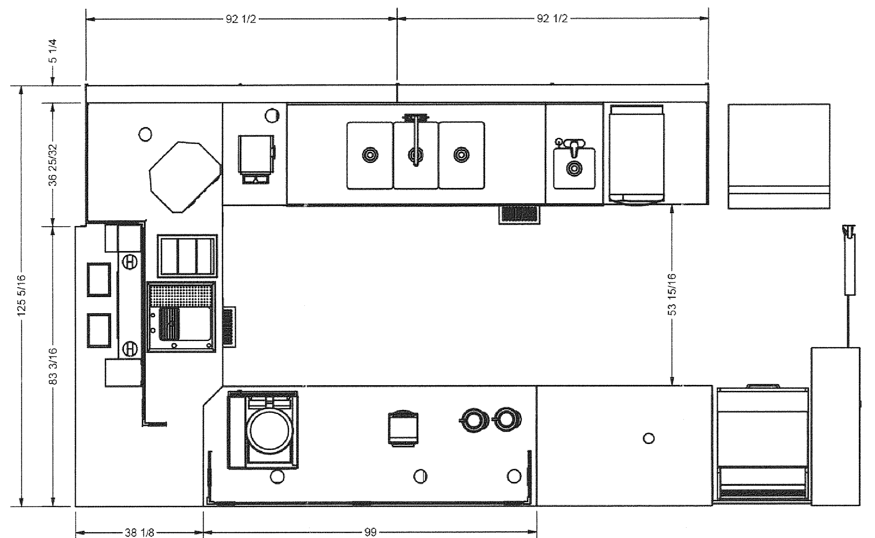
TOP VIEW WITHOUT CANOPY
