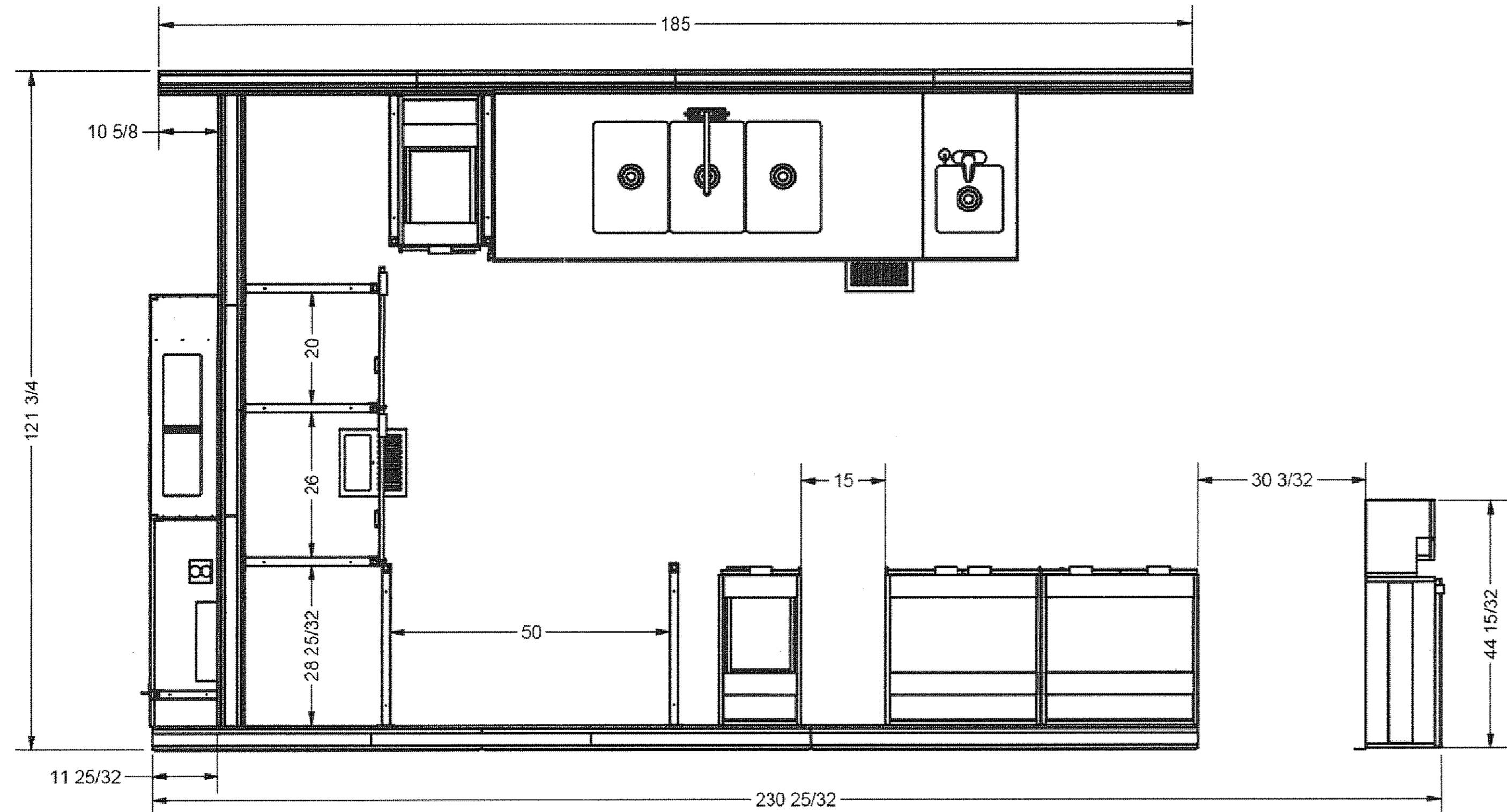
DIEWALL LAYOUT
