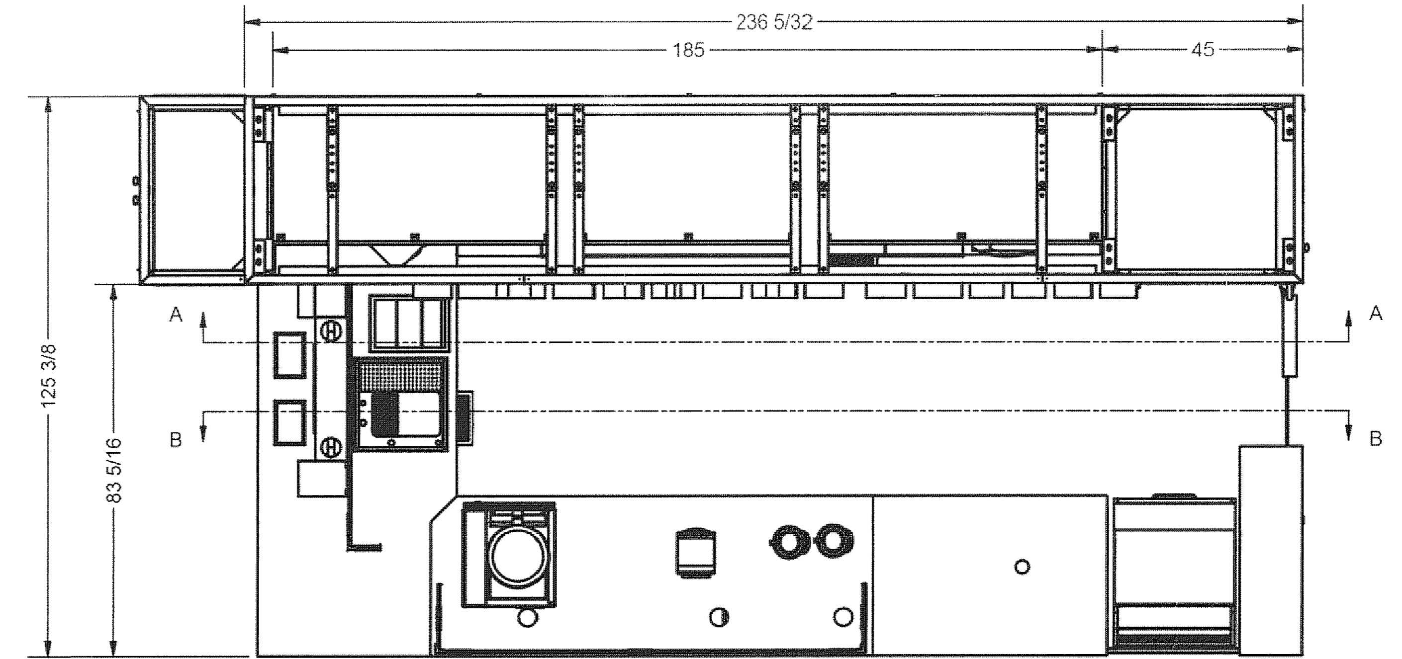
TOP VIEW
