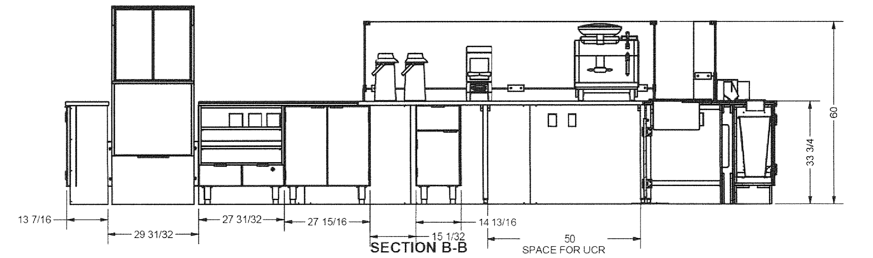
SECTION B-B
